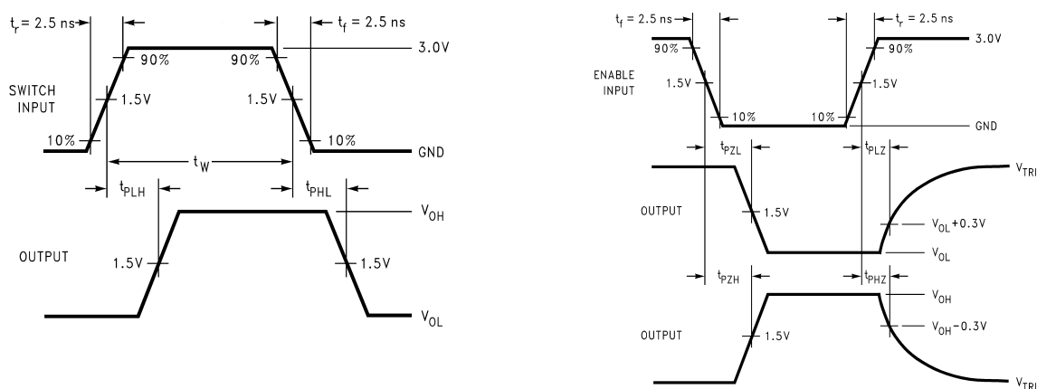
FIGURE 2. AC Waveforms
