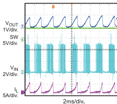
Short Circuit
