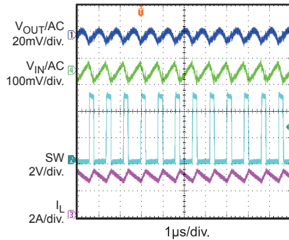
Input and Output Ripple I_{OUT} = 3A
