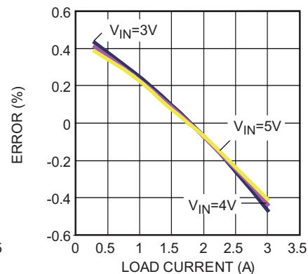
Load Regulation
