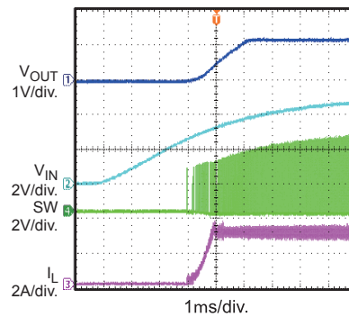
V_{IN} Power Up with 3A Load
