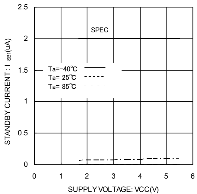
Figure 19. Standby current I_{sB1}(\text{CS}=0\text{V}, \text{ORG}=\text{VCC or OPEN})
