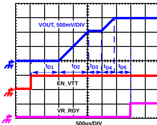
FIGURE 9. SOFT-START WAVEFORMS
