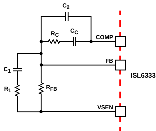
FIGURE 17. COMPENSATION CIRCUIT
