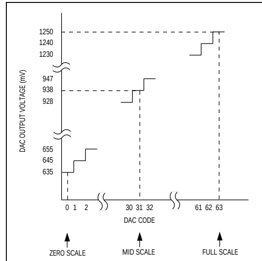
Figure 7. MAX754 LCD DAC Transfer Function
