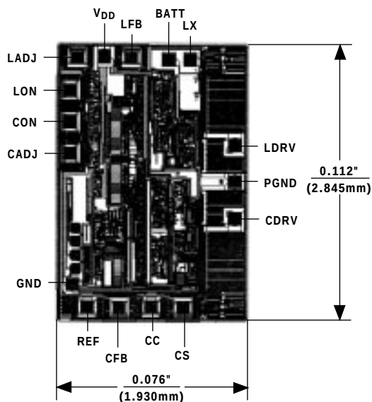
Chip Topography
