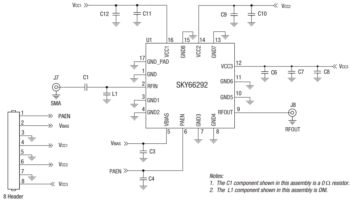
Figure 17. SKY66292-11 Evaluation Board Schematic
