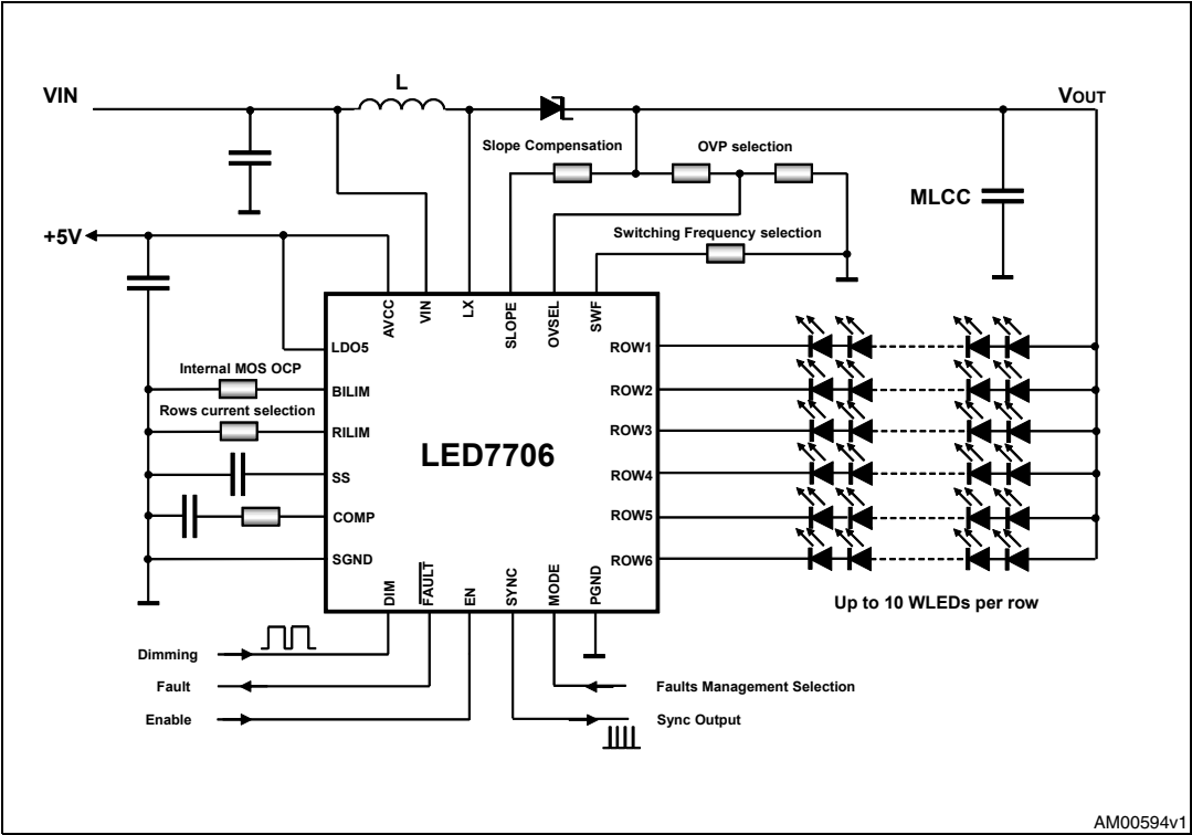
Figure 1. Application circuit
