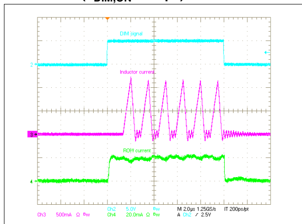
Figure 34. Dimming waveforms ( T_{DIM,ON} = 10 \mu\text{s} )
