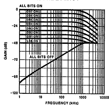
GAIN ( V_{OUT}/V_{REFIN} ) vs FREQUENCY
