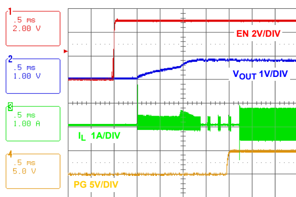
FIGURE 23. SOFT-START WITH PRE-BIASED 1V
