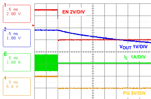
FIGURE 25. SOFT-DISCHARGE SHUTDOWN
