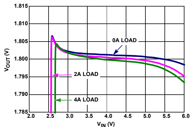
FIGURE 14. OUTPUT VOLTAGE REGULATION vs V_{\text{IN}} (PWM V_{\text{OUT}} = 1.8 )
