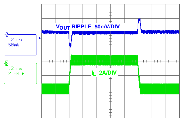
FIGURE 19. LOAD TRANSIENT (PWM)
