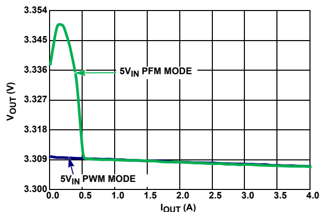
FIGURE 13. V_{\text{OUT}} REGULATION vs LOAD (1MHz, V_{\text{OUT}} = 3.3\text{V} )
