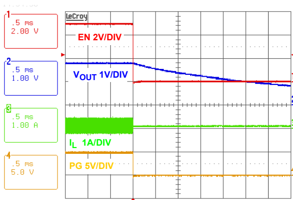
FIGURE 38. SOFT-DISCHARGE SHUTDOWN
