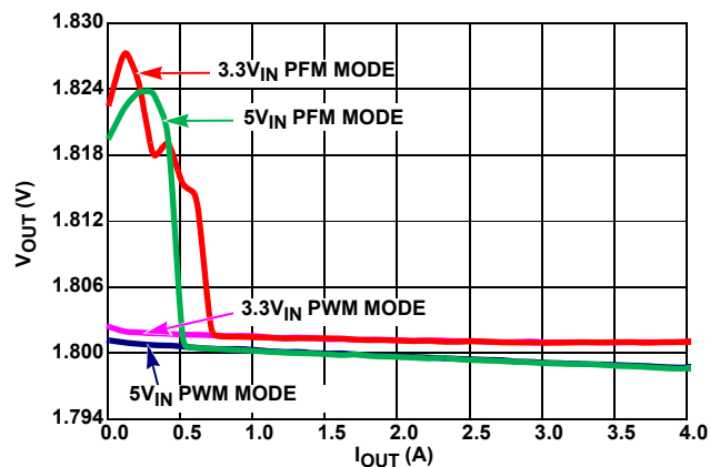
FIGURE 11. V_{\text{OUT}} REGULATION vs LOAD (1MHz, V_{\text{OUT}} = 1.8\text{V} )
