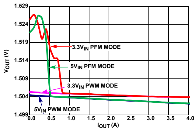
FIGURE 10. V_{\text{OUT}} REGULATION vs LOAD (1MHz, V_{\text{OUT}} = 1.5\text{V} )
