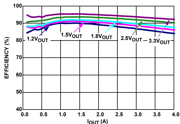
FIGURE 7. EFFICIENCY vs LOAD (1MHz 5 V_{IN} PFM)
