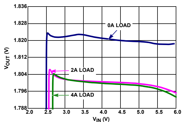
FIGURE 15. OUTPUT VOLTAGE REGULATION vs V_{\text{IN}} (PFM V_{\text{OUT}} = 1.8\text{V} )
