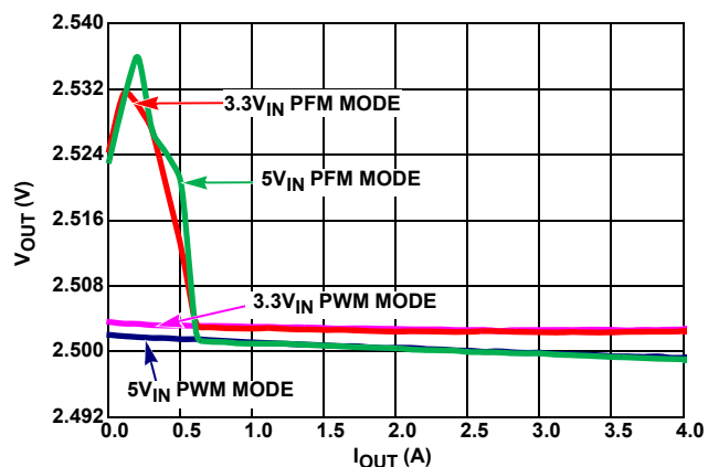
FIGURE 12. V_{\text{OUT}} REGULATION vs LOAD (1MHz, V_{\text{OUT}} = 2.5\text{V} )
