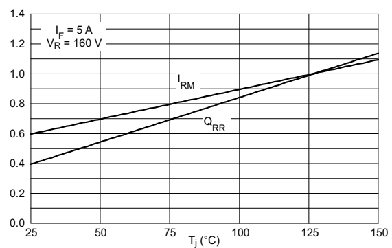
Figure 10. Dynamic parameters versus junction temperature (reference: T_j = 125\text{ °C} )
