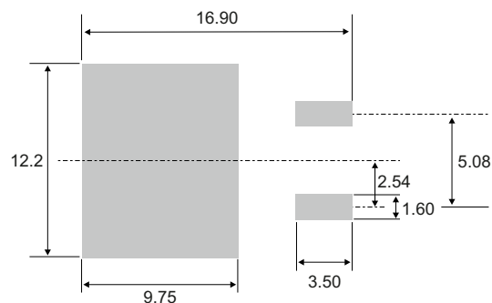
Figure 16. Footprint (dimensions in mm)
