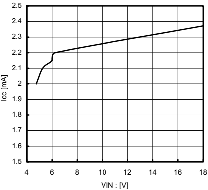
Fig. Circuit Current
