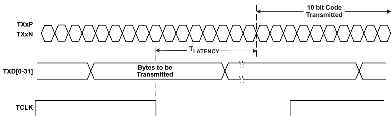
Figure 14. Transmission Latency
