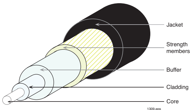
Figure 10. Cross-section of a simple fiber optic cable.
