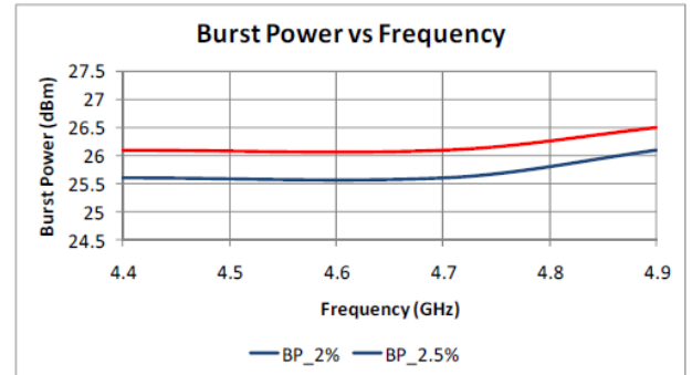
Figure 5 Burst Power
