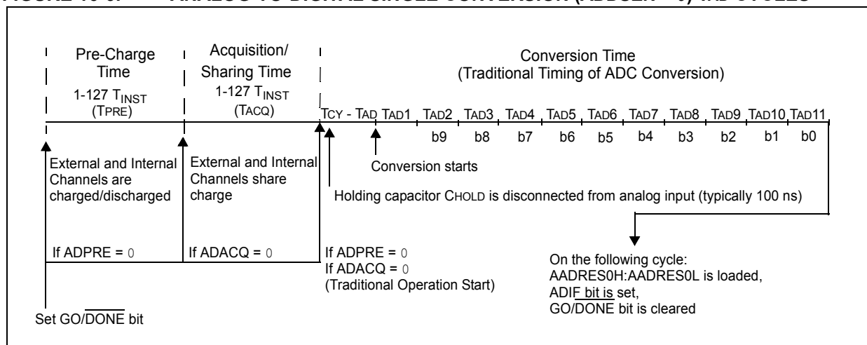
FIGURE 16-6: ANALOG-TO-DIGITAL SINGLE CONVERSION (ADDSEN = 0) T AD CYCLES
