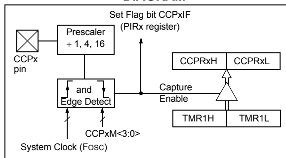
FIGURE 21-1: CAPTURE MODE OPERATION BLOCK DIAGRAM
