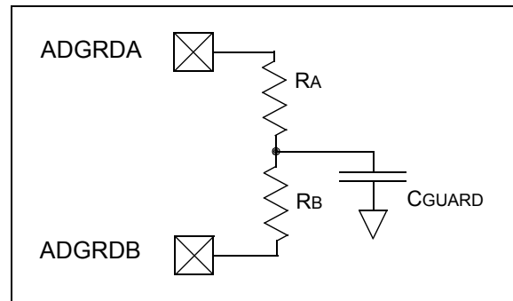
FIGURE 16-11: USER GUARD RING CIRCUIT
