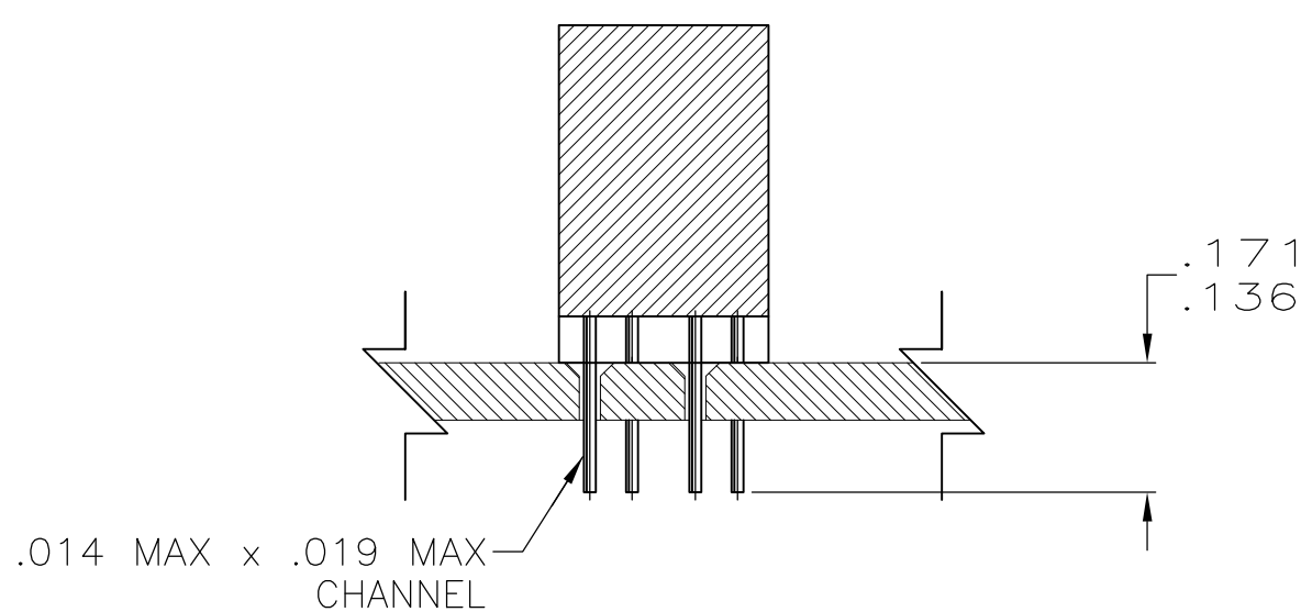
SECTION X-X FLOW SOLDER TYPE
