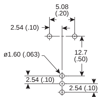
Mounting Holes
