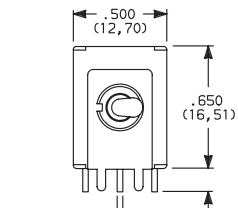
Actuator Shown In Pos. 1 .125 TYP. (3,18) Terminals & Support
