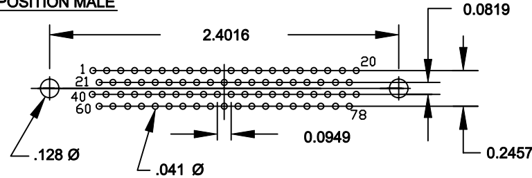
78 POSITION MALE
