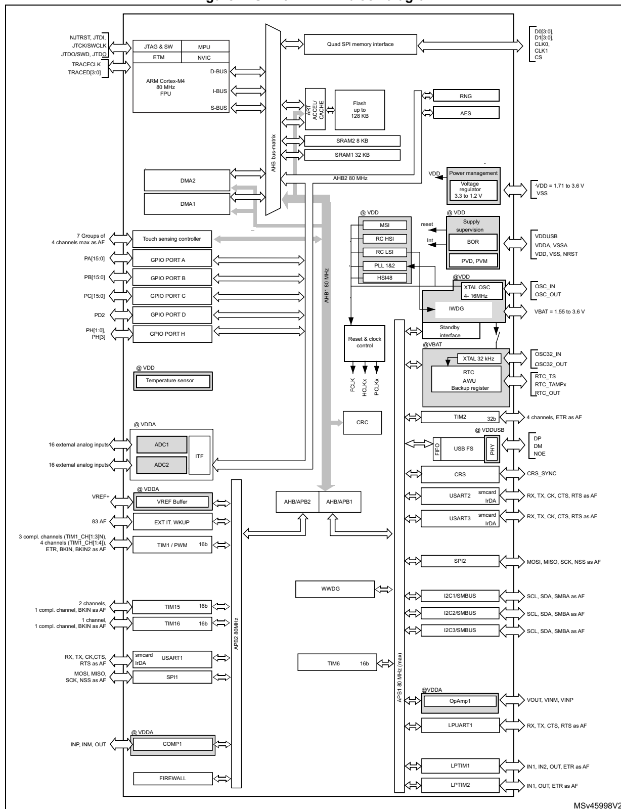
Figure 1. STM32L422xx block diagram
