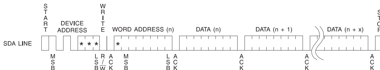
Figure 6. Page Write
