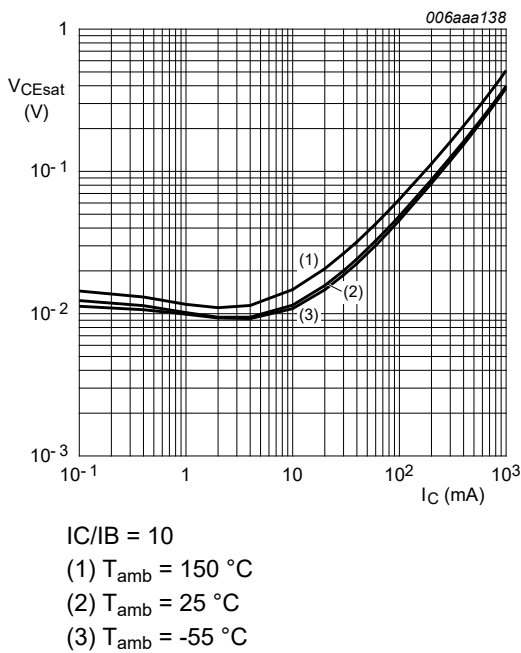
Fig. 10. BC817-25: Collector-emitter saturation voltage as a function of collector current; typical values
