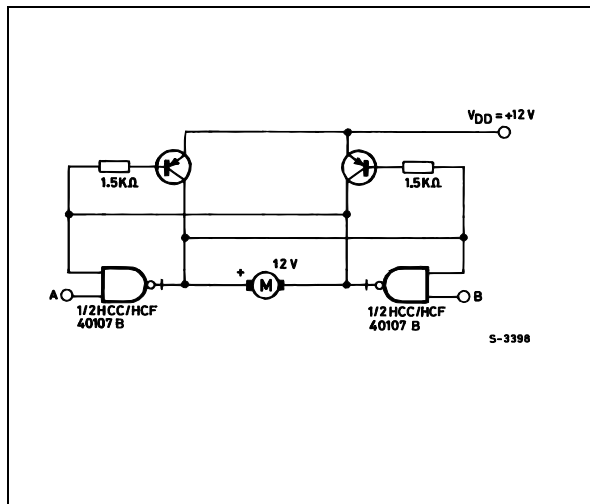
Motor-controller Circuit
