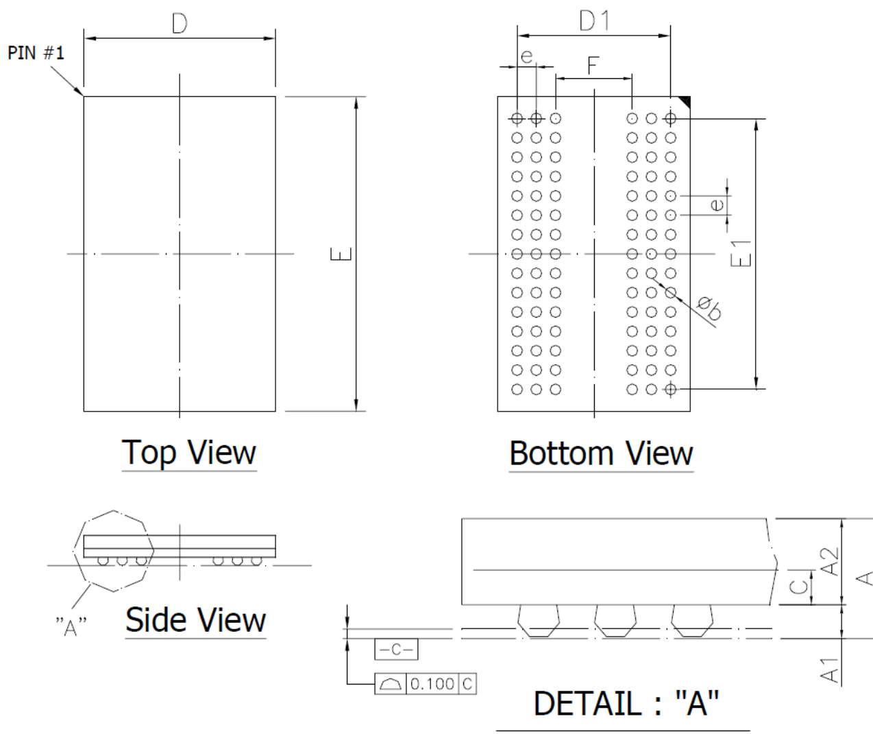
Figure 43. 90 ball FBGA Package 8x13x1.2mm(max.) Outline Drawing Information
