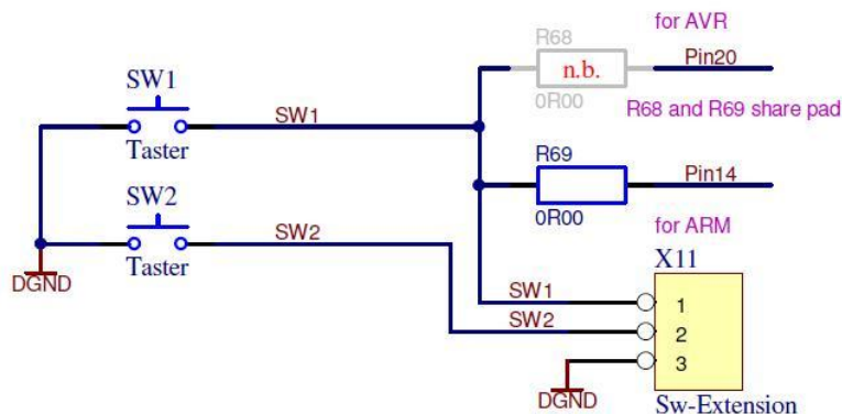
Figure 17: User buttons
