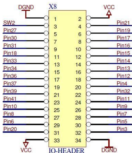
Figure 10: User header
