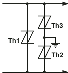
Figure 32. MULTI-POINT PROTECTION
