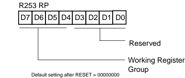
Figure 12. Register Pointer Register
