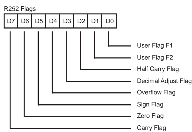
Figure 29. Flag Register (FC H : Read/Write)
