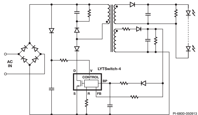
Figure 1. Typical Schematic.
