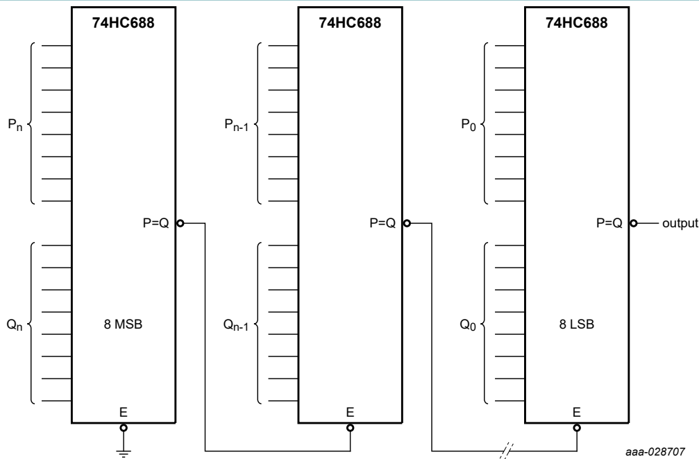
Fig. 7. Binary or BCD comparator
