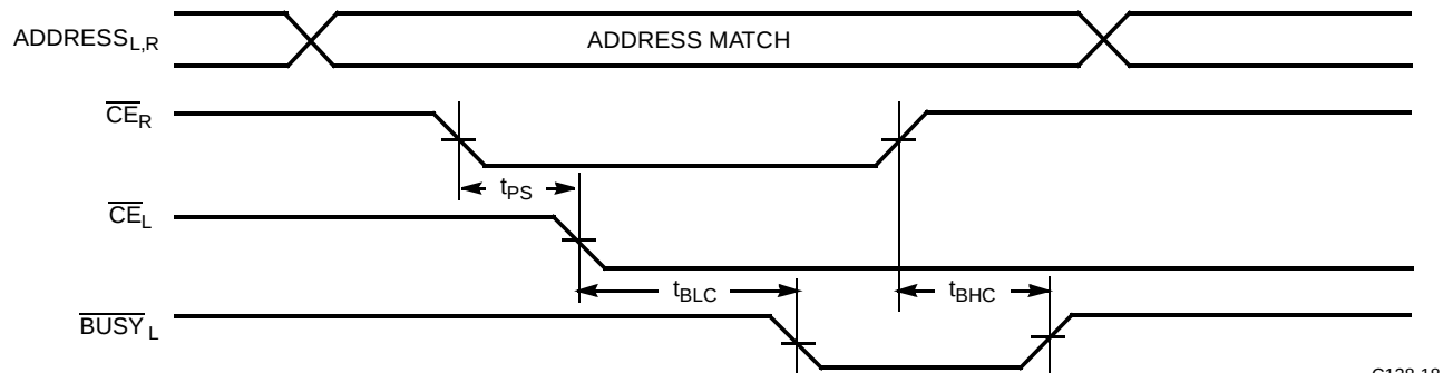
Busy Timing Diagram No. 2 (Address Arbitration) [29]
