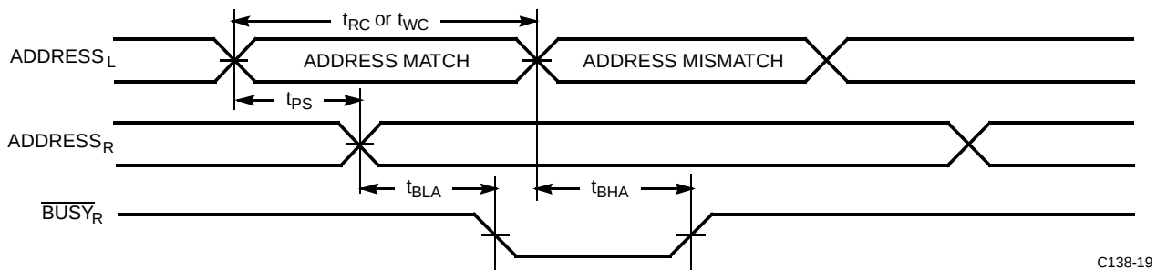
Busy Timing Diagram No. 2 (Address Arbitration) [29]
