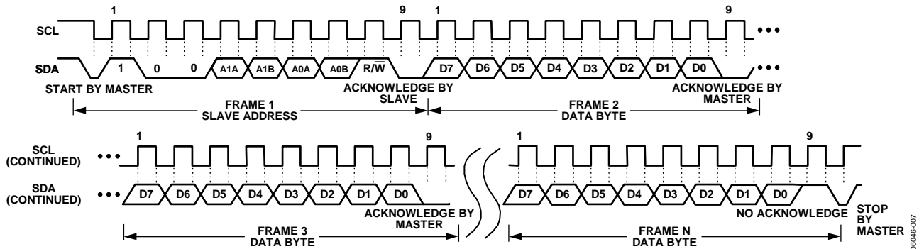
Figure 33. General I2C Read Timing Diagram
