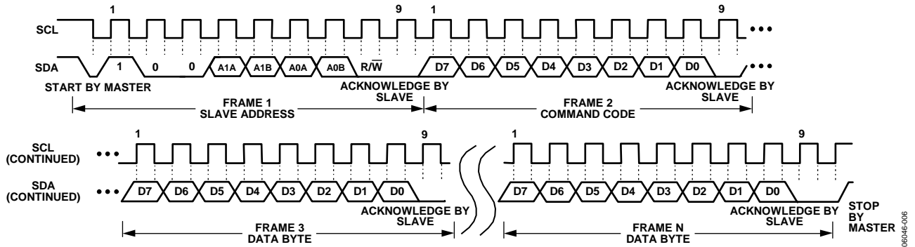
Figure 32. General I2C Write Timing Diagram
