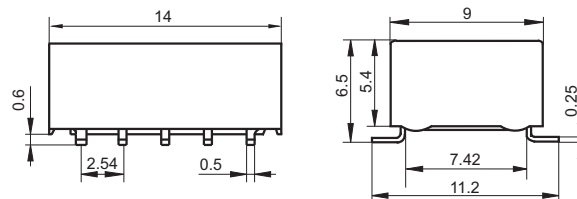
Standard SMT type
