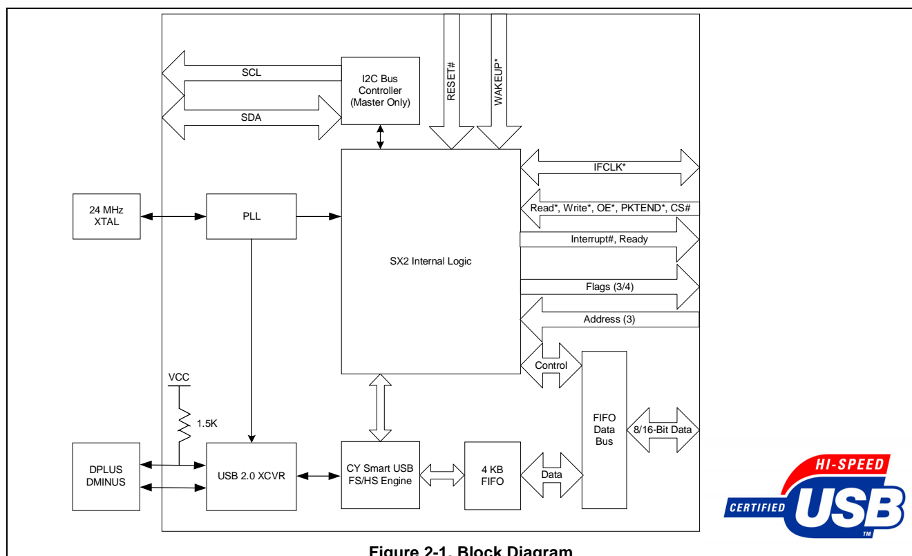
Figure 2-1. Block Diagram
