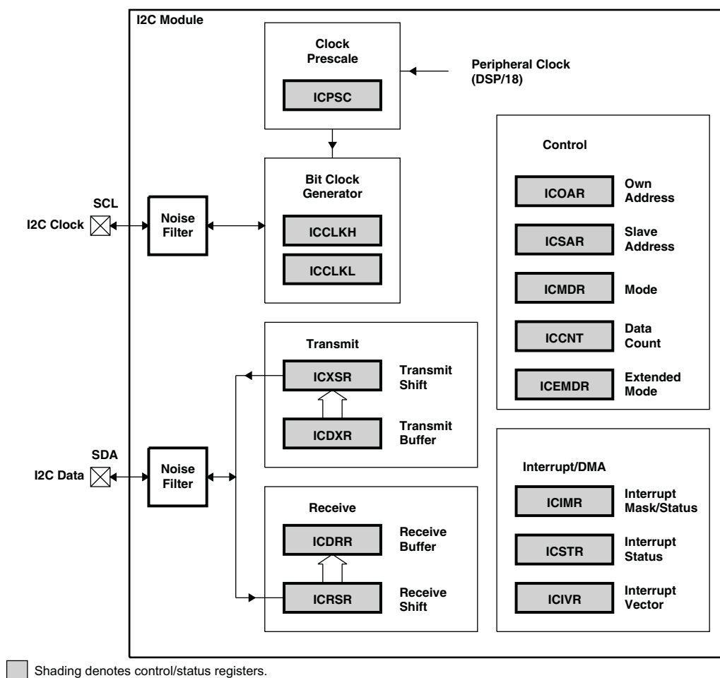
Figure 6-29. I2C Module Block Diagram
