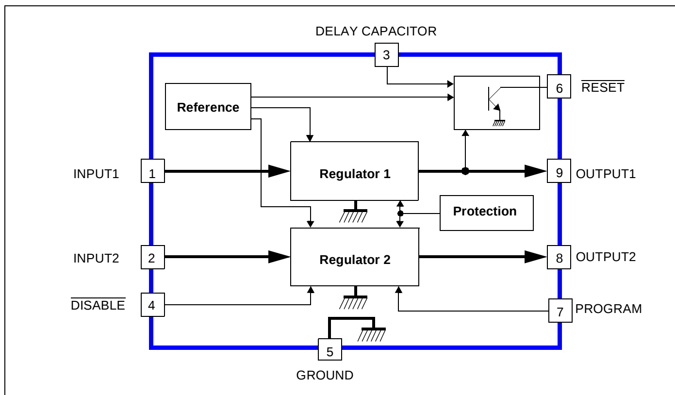
Figure 1: STV8130A# Block Diagram
