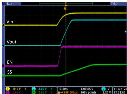
Figure 14. Ramp V_{IN} to Start Up Buck With External 22-nF SS Capacitor
