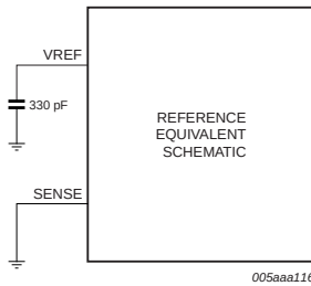
Fig 18. Internal reference, 2 V (p-p) full-scale
