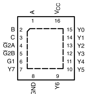
Figure 3-2. SN74AHCT138 RGY Package (Top View)
