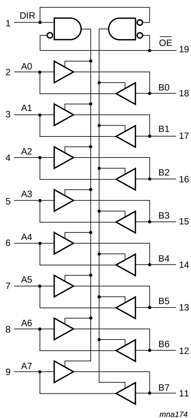
Fig 1. Logic diagram
