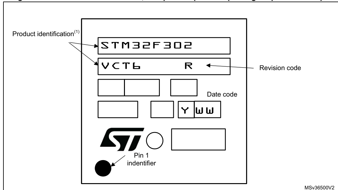
Figure 41. LQFP100 – 14 x 14 mm, low-profile quad flat package top view example
