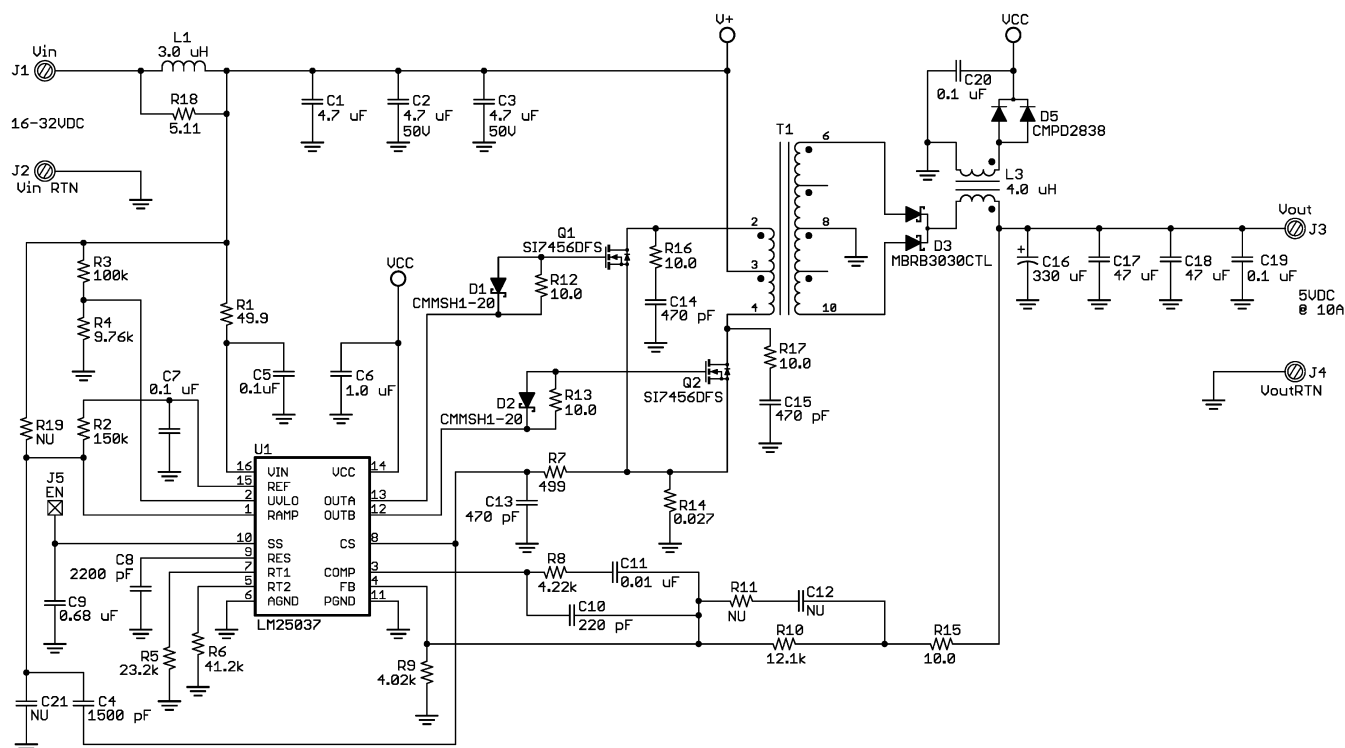
Figure 27. Schematic
