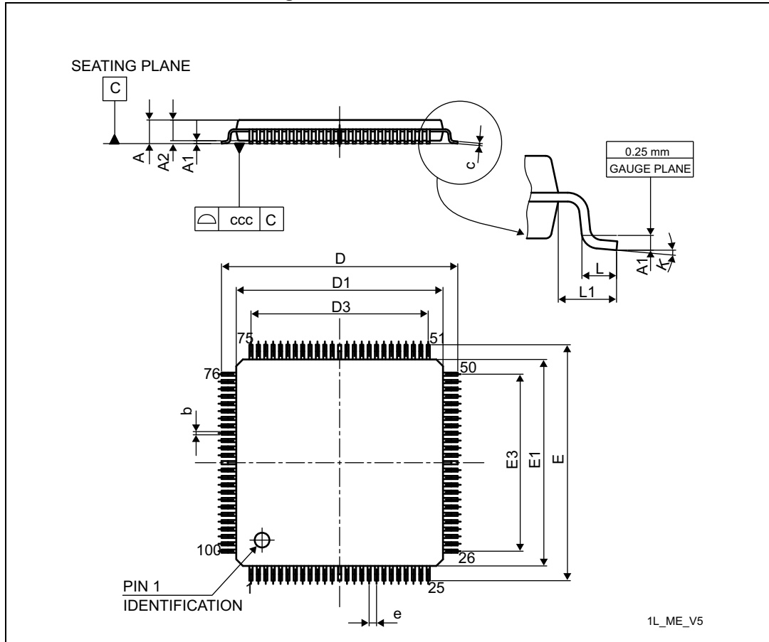
Figure 81. LQFP100 outline
