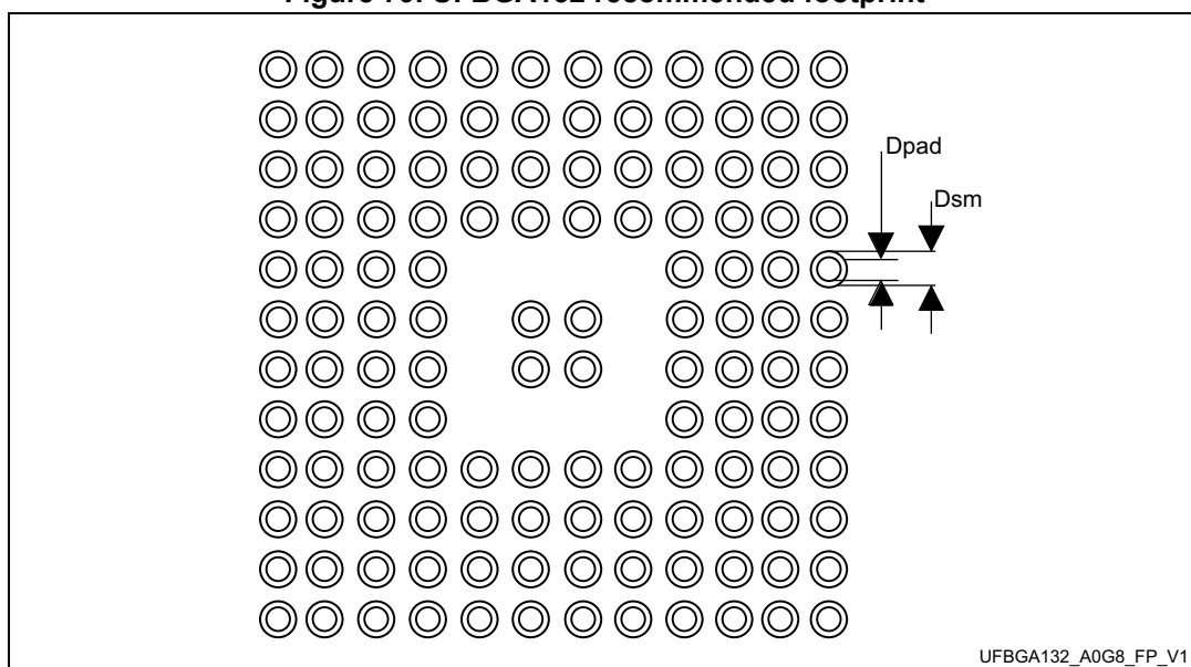
Figure 79. UFBGA132 recommended footprint
