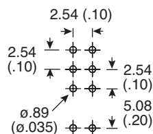
P.C. MOUNTING
