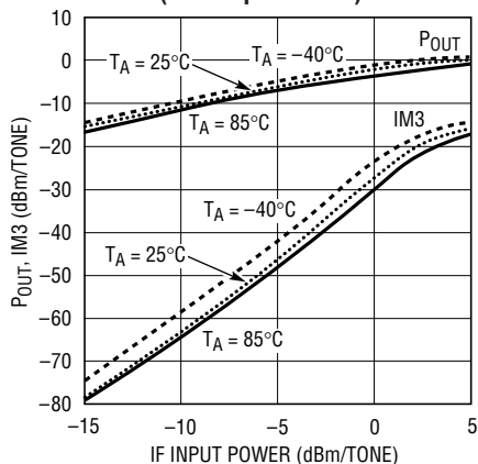
RF Output Power and 3rd Order Intermodulation vs IF Input Power (Two Input Tones)
