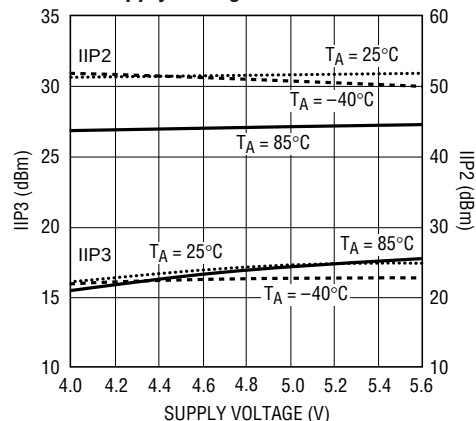
IIP3 and IIP2 vs Supply Voltage
