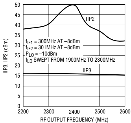
IIP3 and IIP2 vs Output Frequency (Figure 6)
