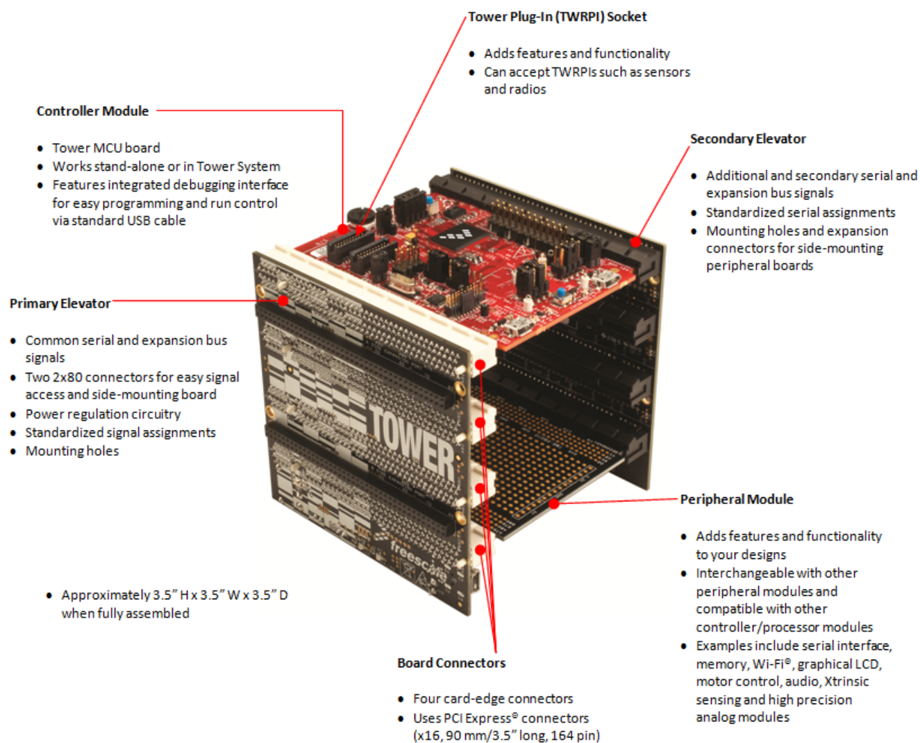
Figure 1. Freescale tower system overview
