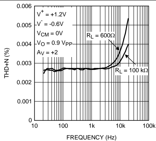
Figure 30. THD+N vs. Frequency
