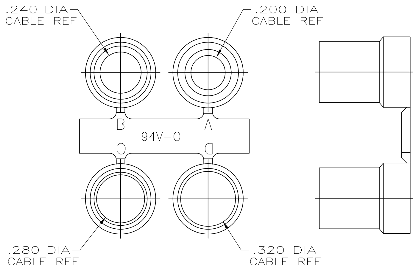
GROMMET ASSORTMENT FOR SIZES 1 & 2 ONLY
