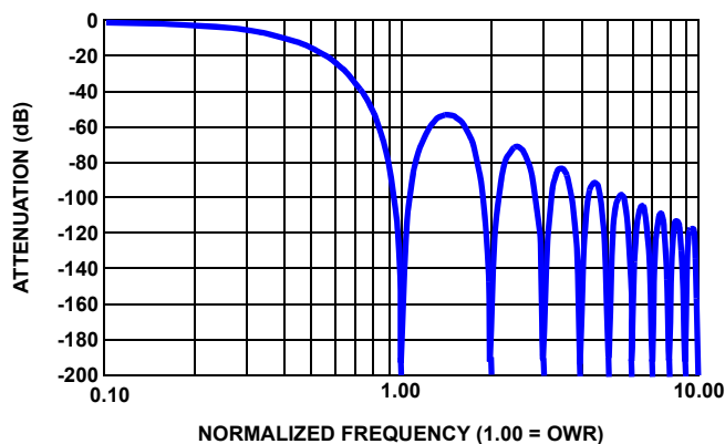
FIGURE 9. TRANSFER FUNCTION OF SINC 4 NORMALIZED TO 1 = OUTPUT WORD RATE
