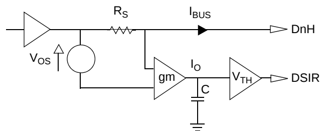
Figure 11. Receive Filter
