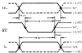
(a) Address and Data Set-up Time and Hold Time, Write Pulse Width (unpulsed \overline{WE} = Low)
