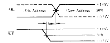
(e) Output Latch Timing, Address Hold Time (unpulsed \overline{WE} = Low)
