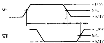
(a) Reset pulse width, \overline{WE} hold time for subsequent writing (address already set-up, unpulsed \overline{WE} = Low)
