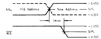
(e) Output Latch Timing, Address Hold Time (unpulsed \overline{WE} = Low)
