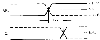
(c) Read Timing, Address Set-up Time (unpulsed \overline{WE} , \overline{OE}_1 , \overline{OE}_2 = Low)
