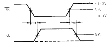
(d) Output Latch Timing, Address Set-up Time (unpulsed \overline{WE} = Low)
